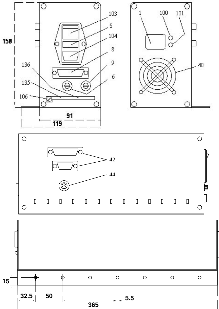
Electronic Control Unit 80.160.00xx - overall dimensions and fitting holes
